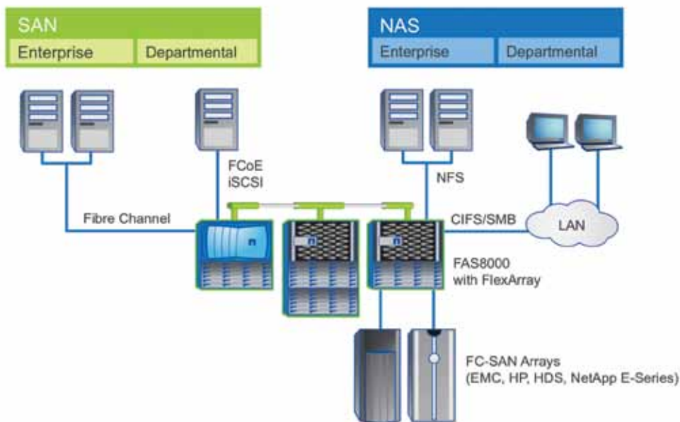
Figure 1) How FlexArray on FAS8000 works.
